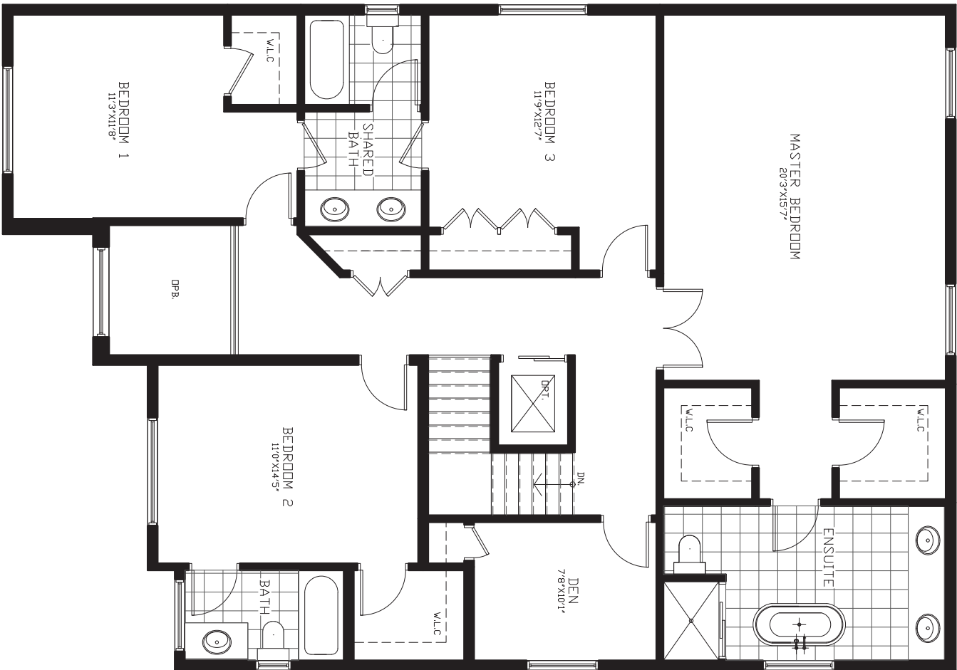
SECOND FLOOR PLAN AREA=1765 SQ.F. INCLUDE DPB. AREA 66 SQ.F.
